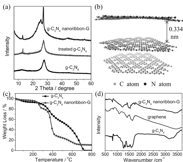
Figure 3. a) XRD patterns of the original \text{g-C}_3\text{N}_4 , treated \text{g-C}_3\text{N}_4 , and \text{g-C}_3\text{N}_4 nanoribbon-G and b) the corresponding structural model of the \text{g-C}_3\text{N}_4 nanoribbon. c) TGA curves of the original \text{g-C}_3\text{N}_4 and \text{g-C}_3\text{N}_4 nanoribbon-G in \text{N}_2 with a heating speed of 10^\circ\text{C min}^{-1} . d) FTIR spectrum of the original \text{g-C}_3\text{N}_4 , graphene and \text{g-C}_3\text{N}_4 nanoribbon-G, respectively.
